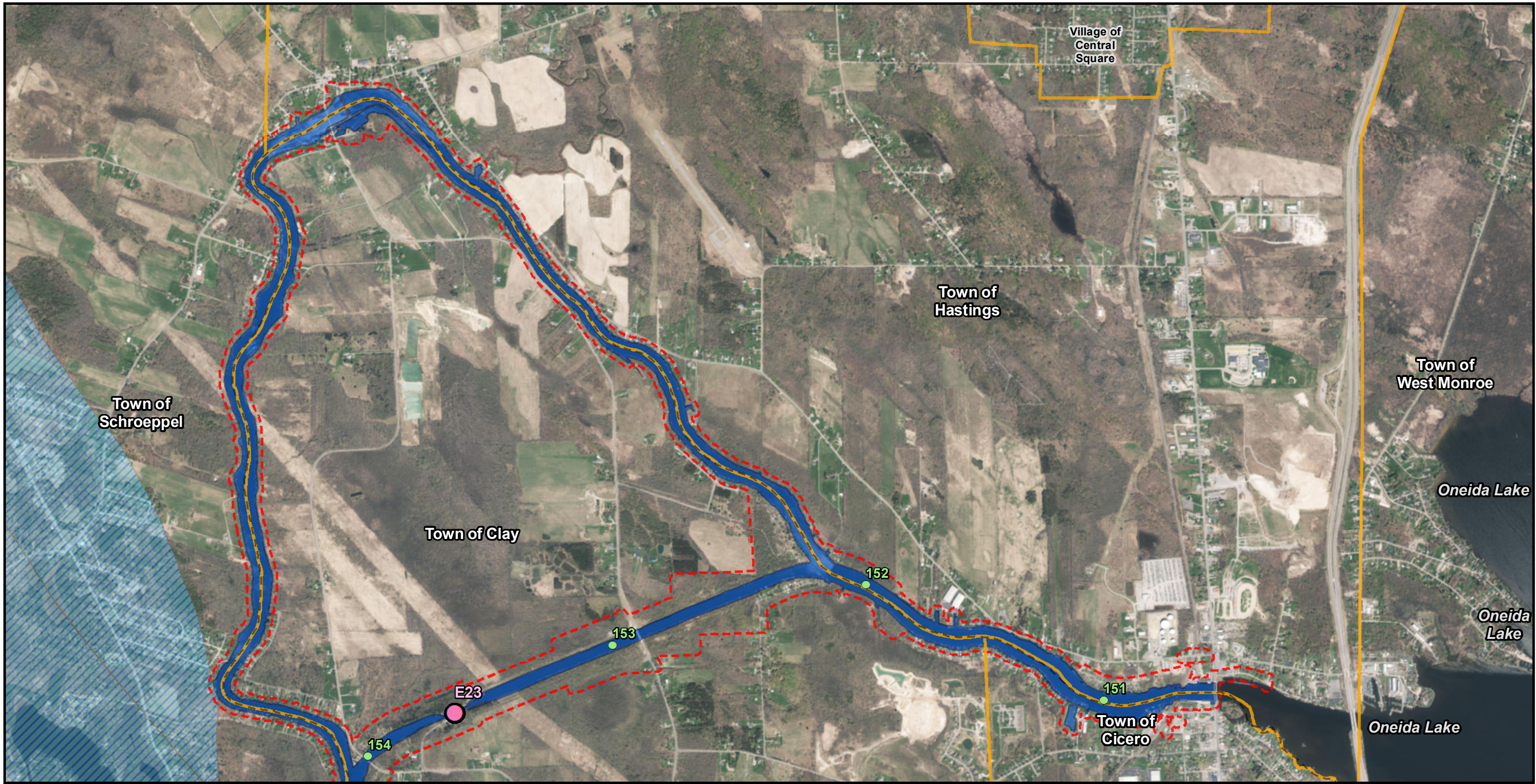
Figure 72F: Aquifers
